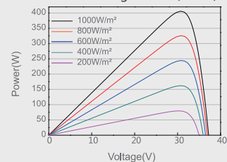
Power-Voltage Curve (405W)
