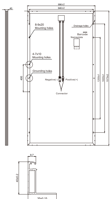
Dimensions of PV Module Unit: mm
